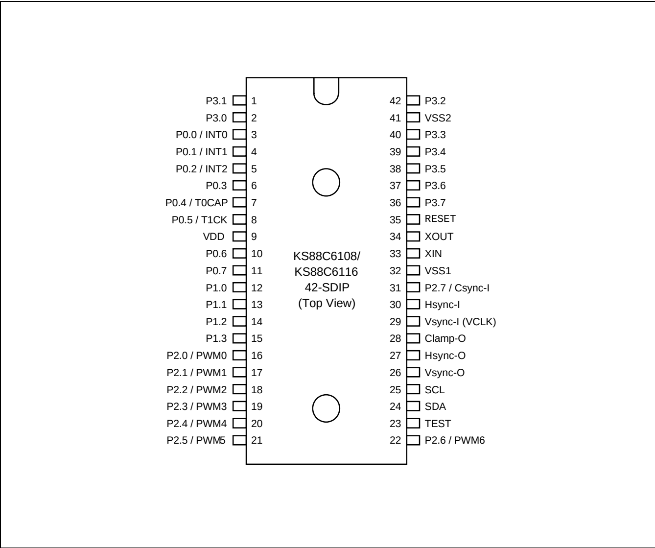
Figure 1-3. Pin Assignment Diagram (42-SDIP Package)
