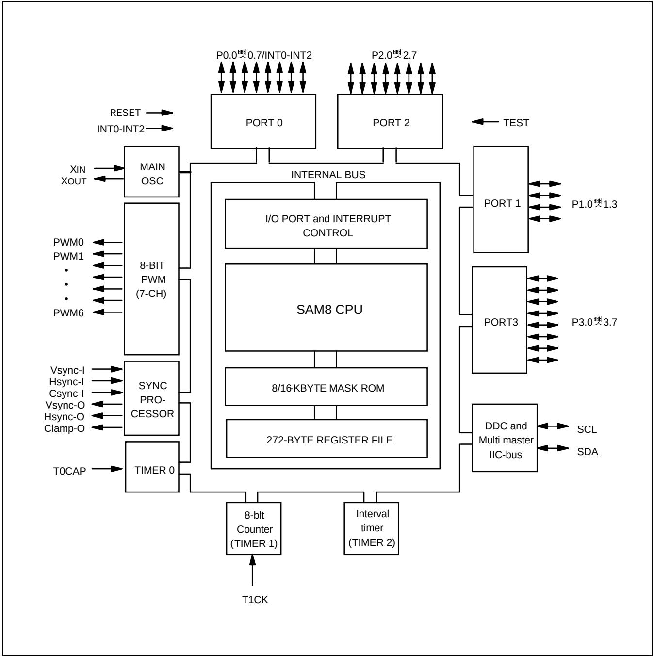
Figure 1-2. Block Diagram
