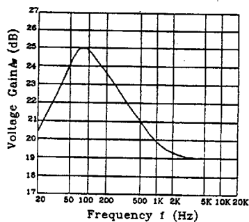
Frequency Response with Base Boost
