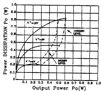
Power Dissipation vs. Output Power ( R_L=8\Omega )
