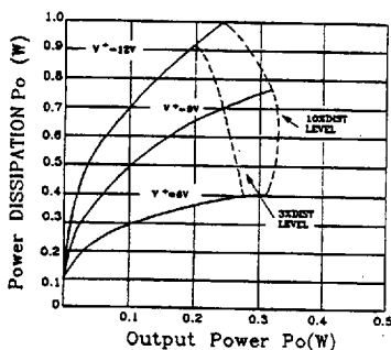
Power Dissipation vs. Output Power ( R_L=4\Omega )
