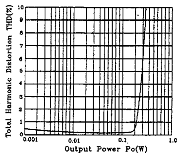
Total Harmonic Distortion vs. Output Power ( V^+=6\text{V}, R_L=8\Omega, f=1\text{KHz} )
