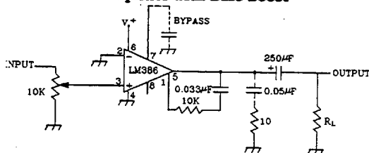
Amplifier 2
