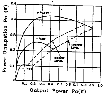
Power Dissipation vs. Output Power ( R_L=16\Omega )
