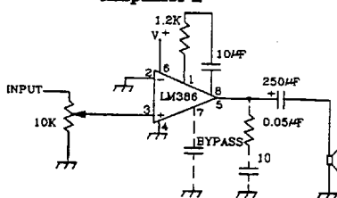
Amplifier 2
