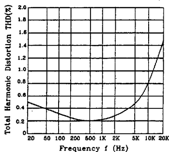
Total Harmonic Distortion vs. Frequency ( V^+=6\text{V}, R_L=8\Omega, P_o=125\text{mW}, A_v=26\text{dB} )
