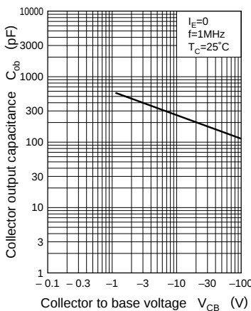
C_{ob} - I_C
