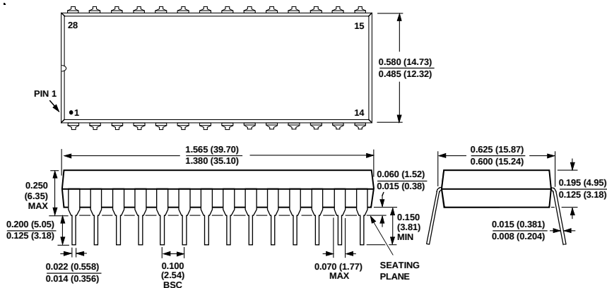
N-28 28-Lead Plastic DIP
