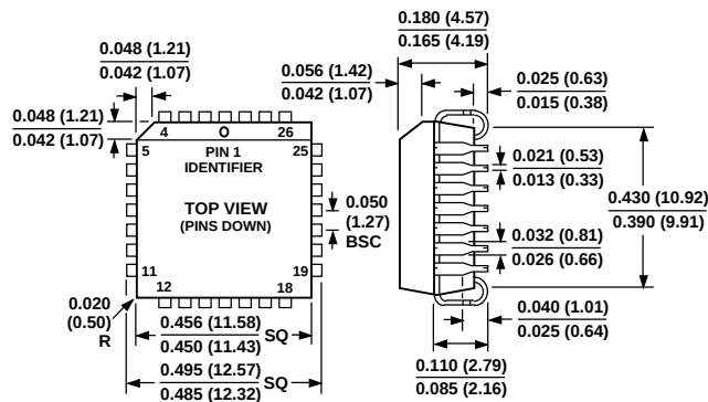
P-28A 28-Lead PLCC
