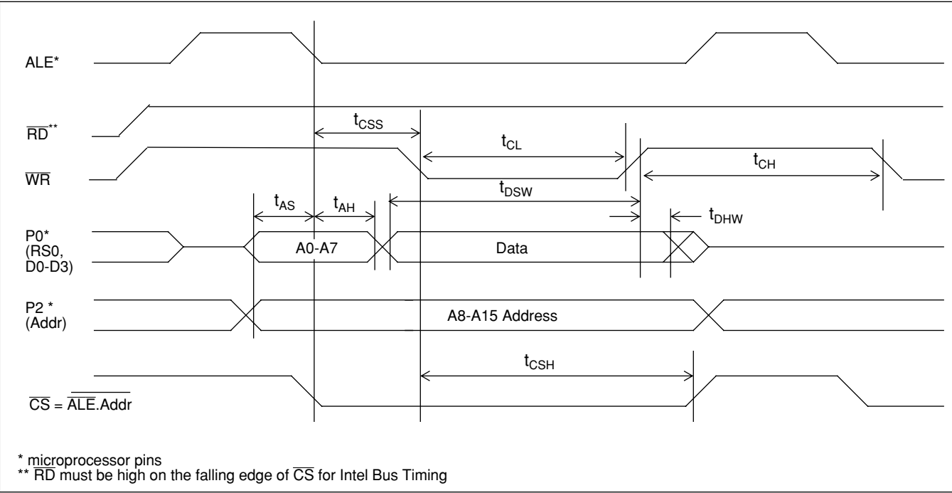
Figure 19 - Intel Write Timing Diagram
