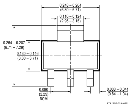
ST Package 3-Lead Plastic SOT-223 (LTC DWG # 05-08-1630)
