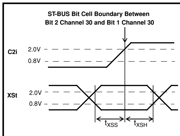
Figure 18 - XSt Timing
