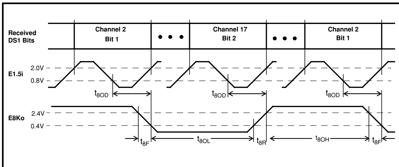
Figure 19 - E8Ko Timing
