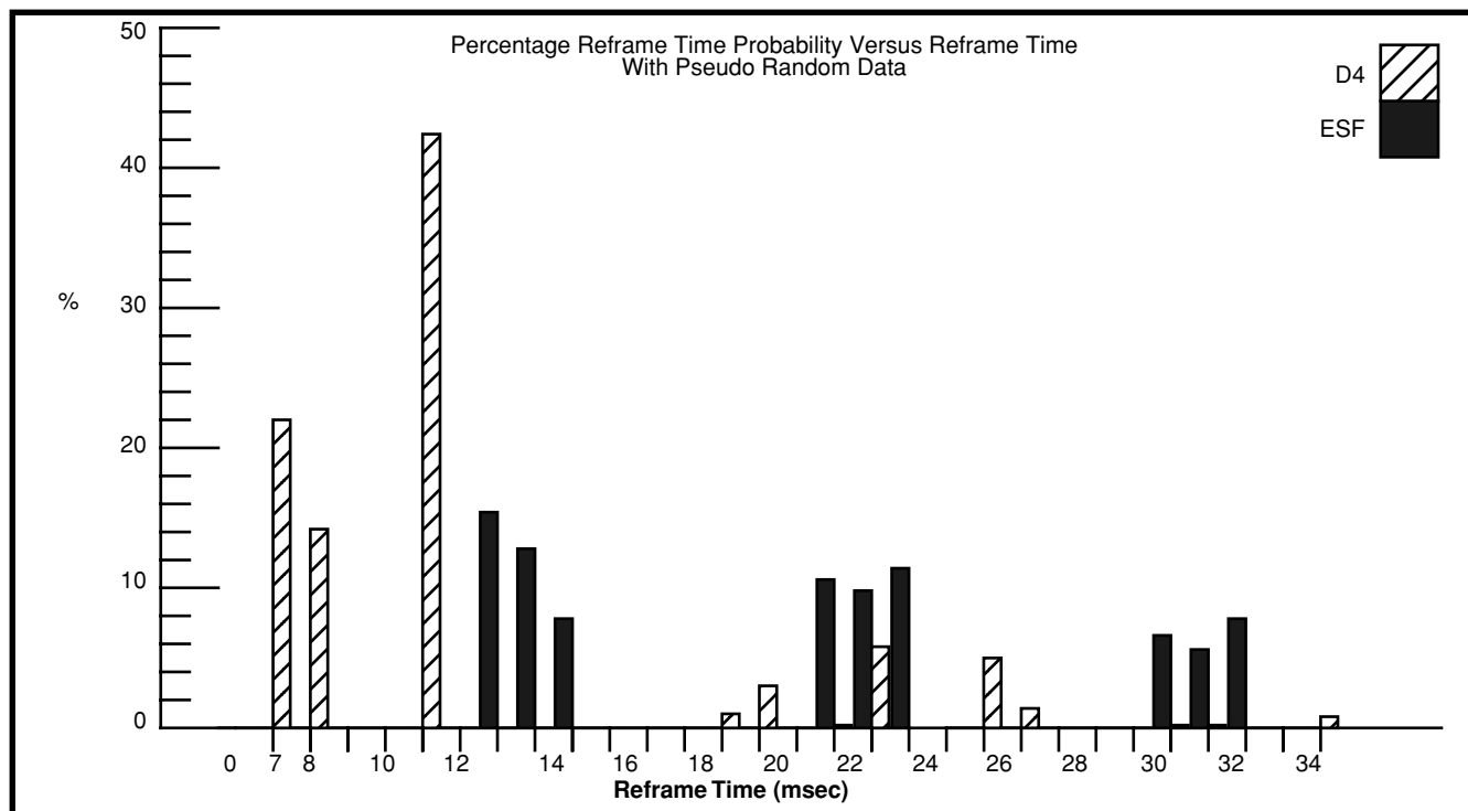
Figure 10 - Reframe Time
