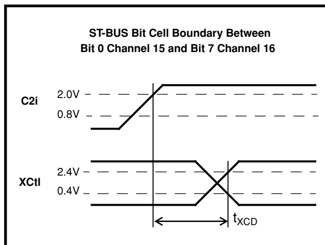
Figure 17 - XcTi Timing
