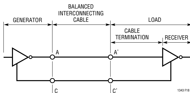
Figure 18. Typical V.28 Interface
