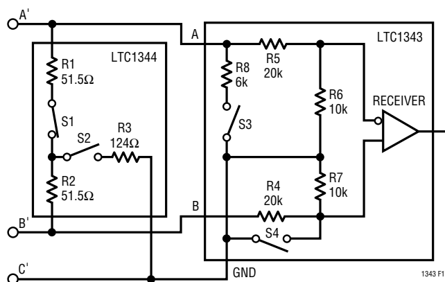
Figure 17. V.11 Receiver Configuration
