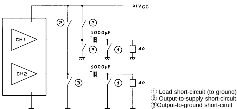
Dual-mode short-circuit test circuit
