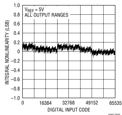
LTC1592 Integral Nonlinearity
