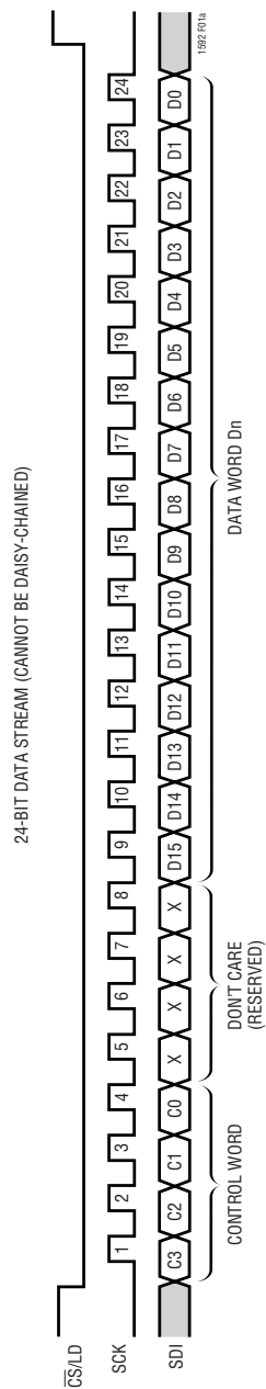
Figure 1a. 24-Bit Load Sequence (Cannot Daisy-Chain Multiple LTC1592s)
