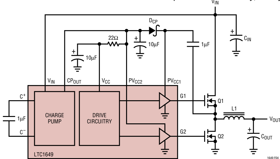
Figure 4. LTC1649 Power Supplies
