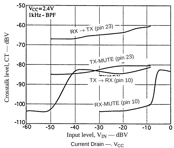
Crosstalk Characteristics
