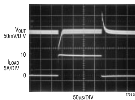
Transient Response, V_{OUT} = 2.8V
