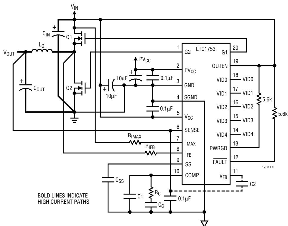
Figure 10. LTC1753 Layout Diagram
