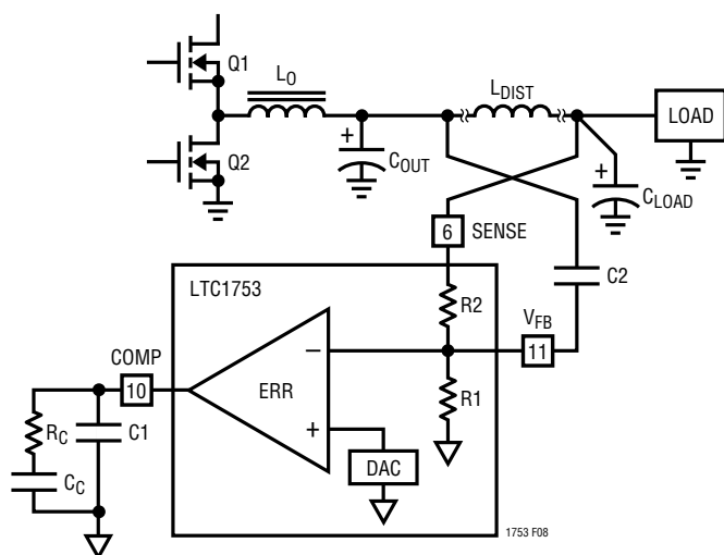
Figure 8. Feedback Connections for Remote Sense Applications
