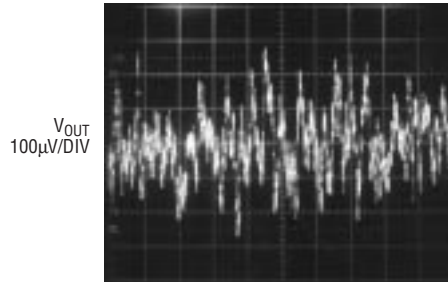
LT1763-5 10Hz to 100kHz Output Noise C_{BYP} = 100\text{pF}
