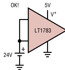
INPUT OVERVOLTAGE
