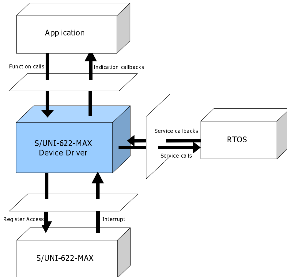
Figure 1. Interfaces of the S/UNI-622-MAX Driver
