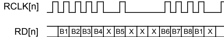
Figure 16 – Unchannelised Receive Link Timing
