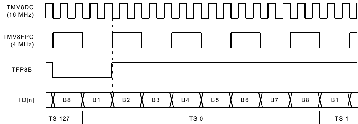
Figure 14 – Transmit 8.192 Mbps H-MVIP Link Timing
