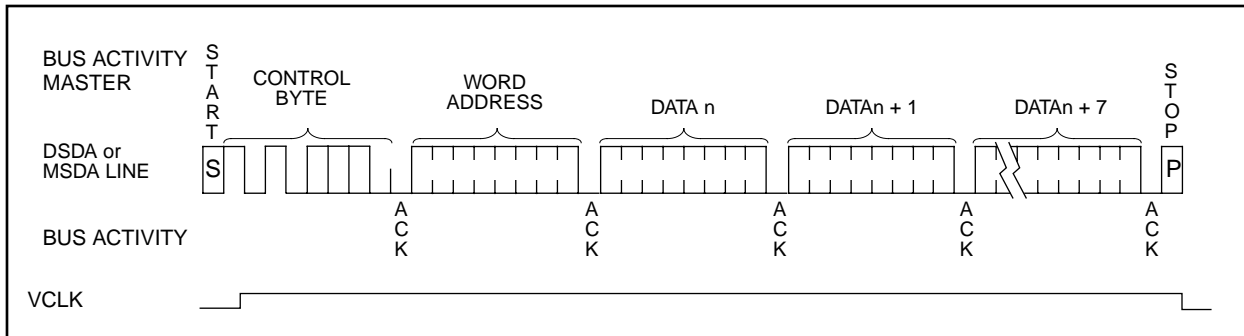
FIGURE 4-2: PAGE WRITE
