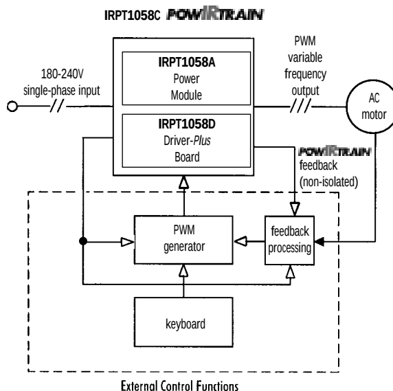
Figure 2. The IRPT1058C POWERTRAIN within a motor control system
