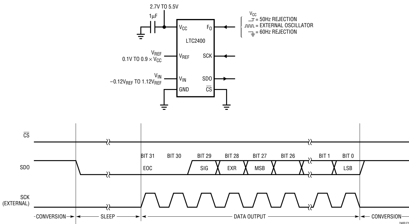
Figure 13. External Serial Clock, \overline{CS} = 0 Operation
