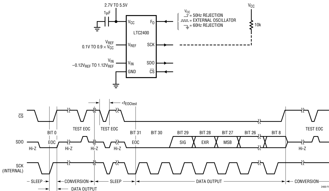
Figure 11. Internal Serial Clock, Reduced Data Output Length
