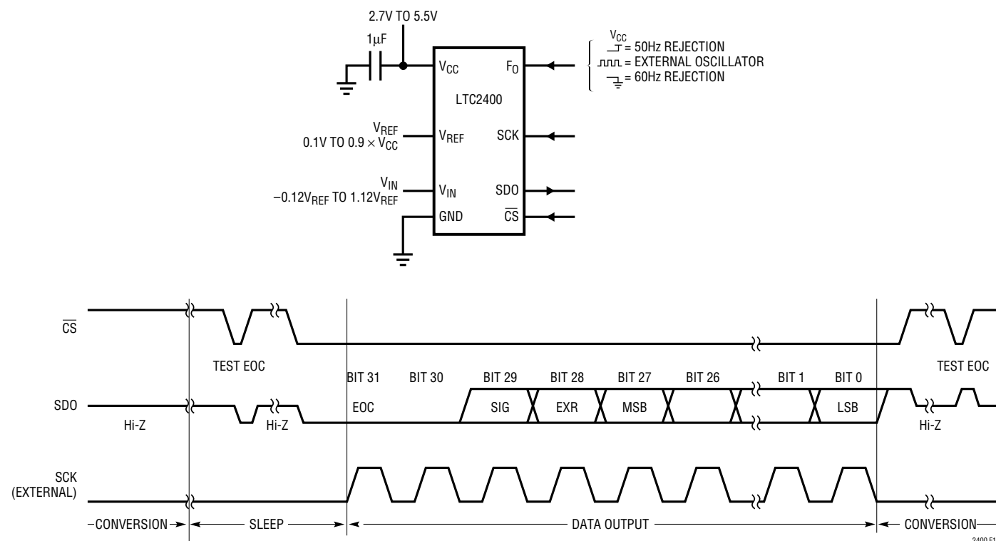
Figure 14. External Serial Clock, Single Cycle Operation
