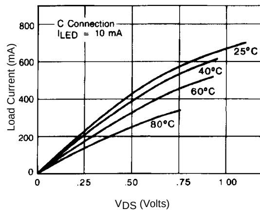
Figure 4. Typical On-Characteristics (C Connection)
