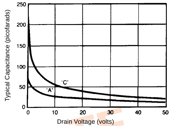
Figure 10. Typical Output Capacitance
