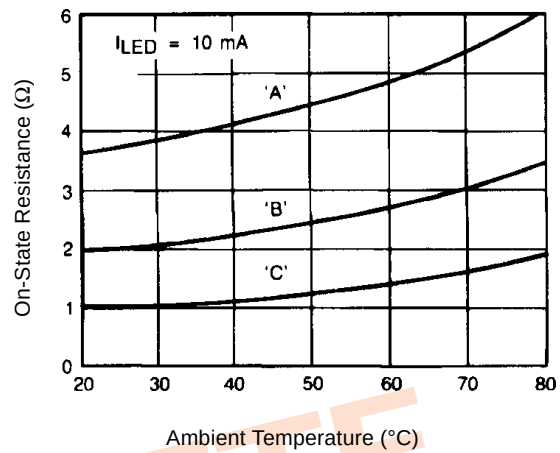
Figure 2. Typical On-Resistance
