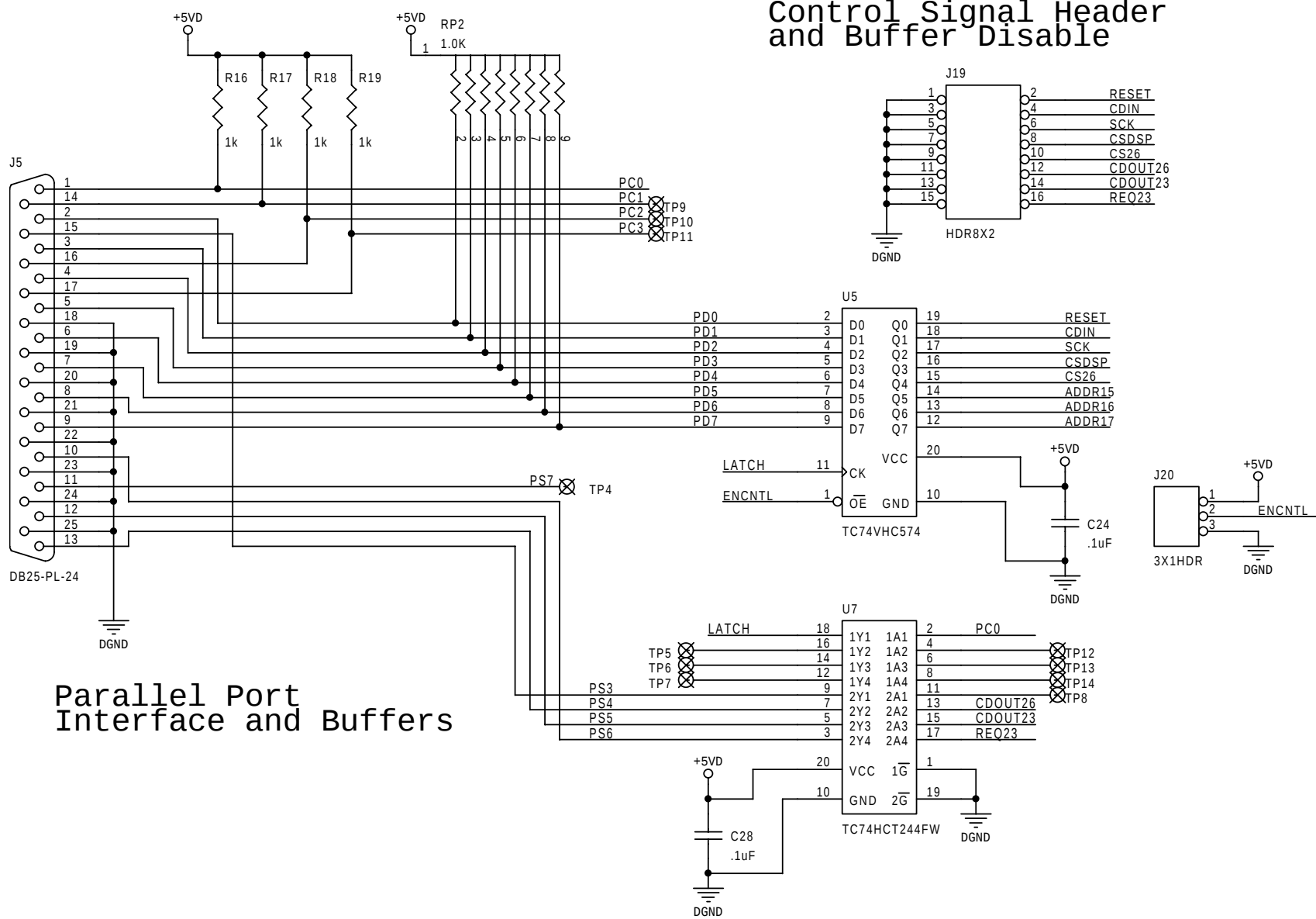
Figure 2. Control Interface
