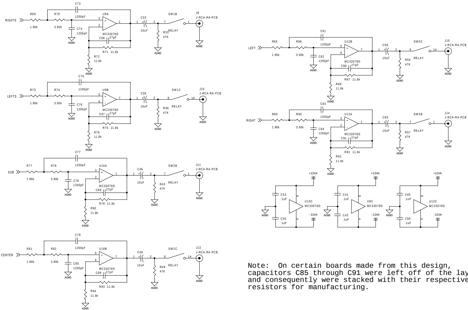
Figure 6. Analog Output
