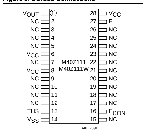
Figure 3. SOIC28 Connections
