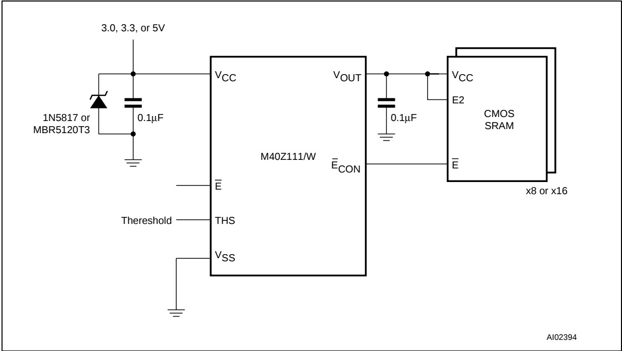
Figure 4. Hardware Hookup
