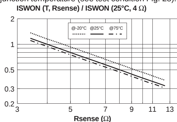
Fig. 26: Typical relative variation of switching-on current (positive or negative) versus R_{SENSE} resistor and junction temperature (see test condition Fig. 28).
