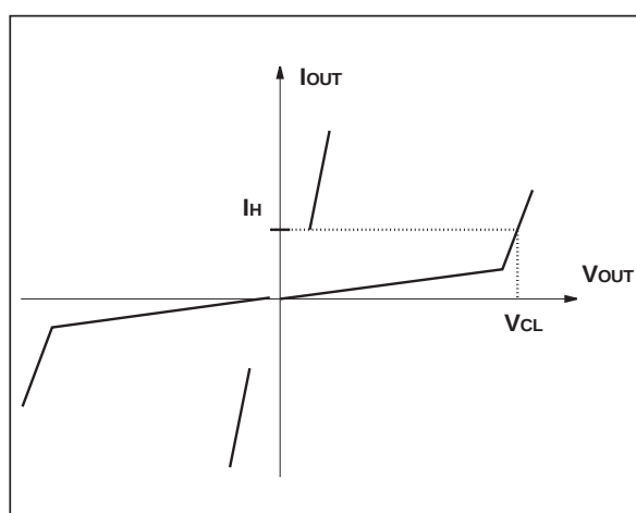
Fig. 2: ACS102 switch static characteristic.
