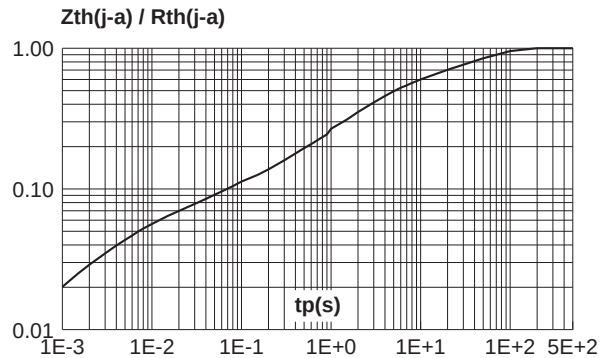
Fig. 7-2: Relative variation of thermal impedance junction to ambient versus pulse duration (printed circuit board FR4, e(Cu) = 35\mu m , S(Cu) = 40mm^2 under "com" pins) (ACS102-5T1) (SO-8).
