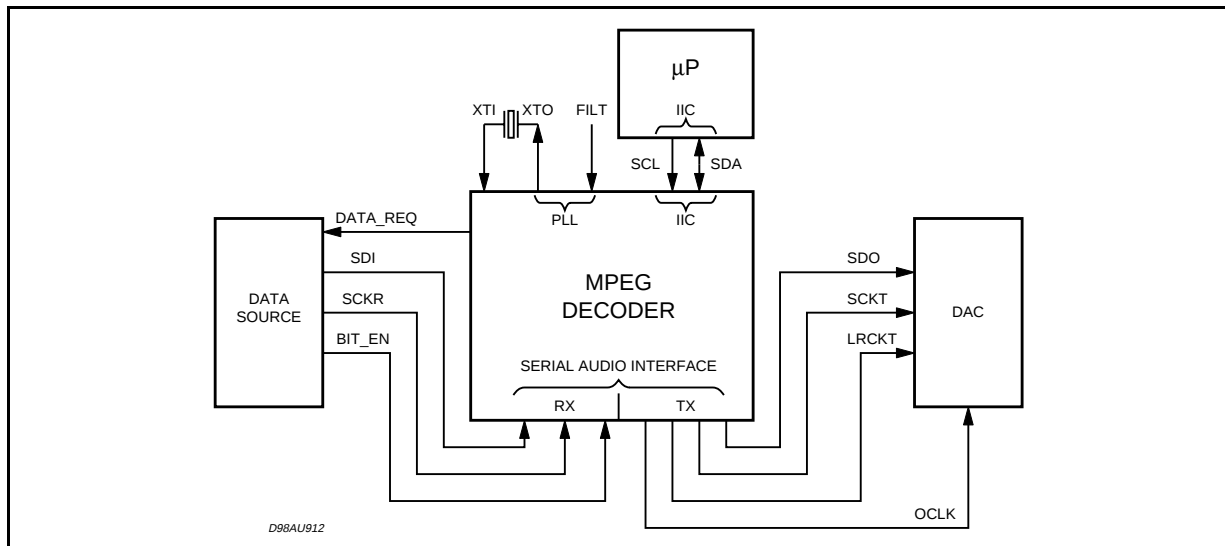
Figure 7. MPEG Decoder Interfaces.
