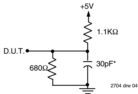
Figure 2. Output Load
