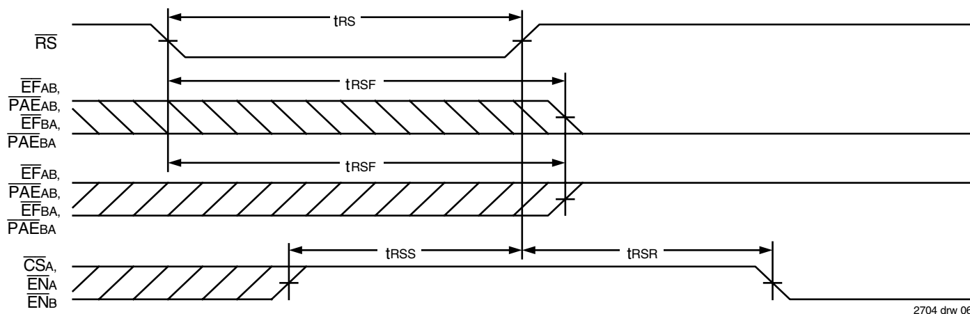
Figure 3. Reset Timing
