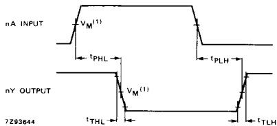
Fig. 13 Waveforms showing the input (nA) to output (nY) propagation delays and the output transition times.
