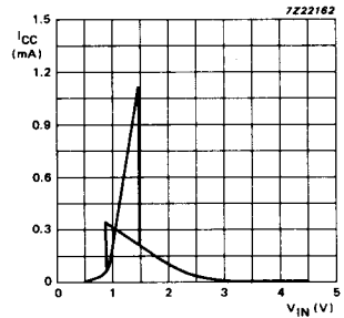
Fig. 11 Typical HCT transfer characteristics; V_{CC} = 4.5 \text{ V} .
