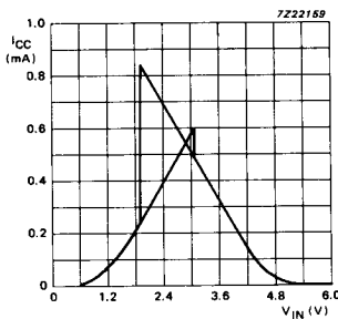
Fig. 10 Typical HC transfer characteristics; V_{CC} = 6 \text{ V} .
