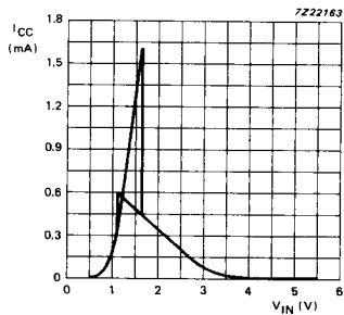
Fig. 12 Typical HCT transfer characteristics; V_{CC} = 5.5 \text{ V} .
