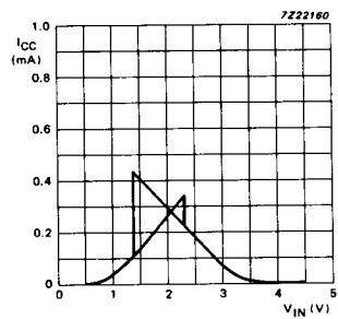
Fig. 9 Typical HC transfer characteristics; V_{CC} = 4.5 \text{ V} .
