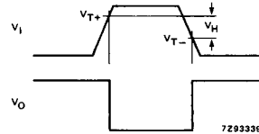
Fig. 7 Waveforms showing the definition of V_{T+} , V_{T-} and V_H ; where V_{T+} and V_{T-} are between limits of 20% and 70%.
