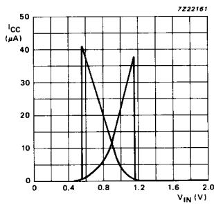
Fig. 8 Typical HC transfer characteristics; V_{CC} = 2 \text{ V} .
