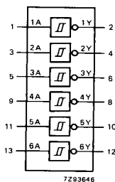
Fig. 4 Functional diagram.
