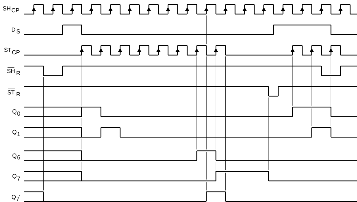
Fig.6 Timing diagram.
