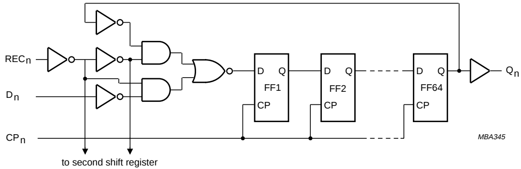
Fig.3 Logic diagram.
