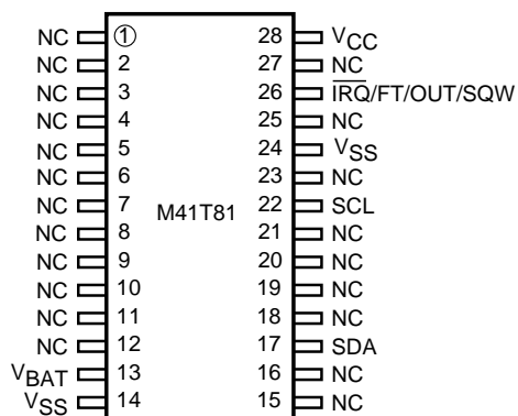
Figure 5. 28-pin, 300mil SOIC (MX) Connections
