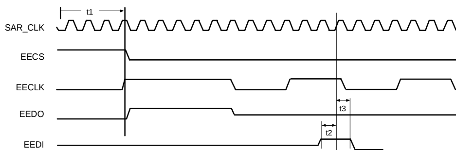
Figure 9 EEPROM Timing
