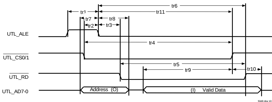
Figure 5 Utility Bus Read Cycle
