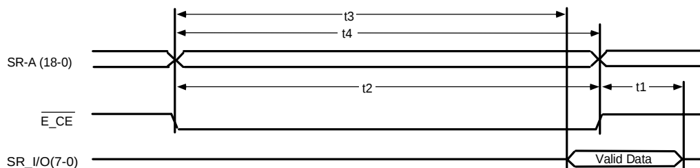
Figure 8 EPROM Timing
