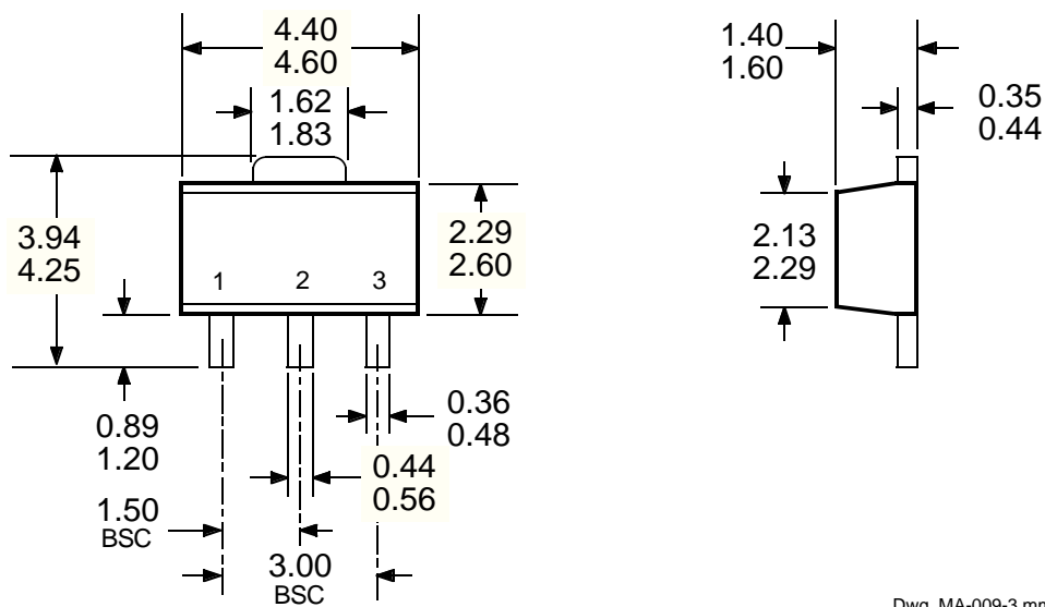
Dimensions in Millimeters (controlling dimensions)
