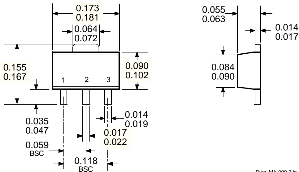
Dimensions in Inches (for reference only)
