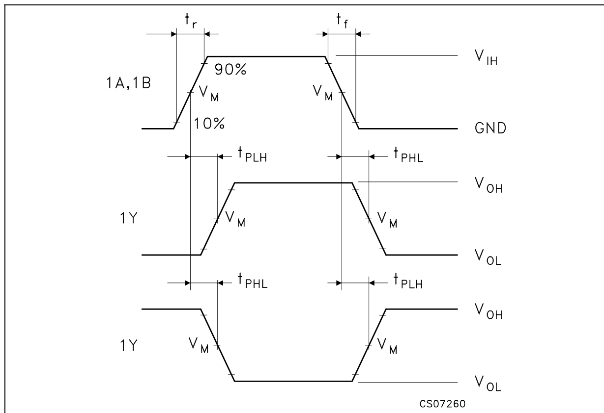
WAVEFORM: PROPAGATION DELAY ( f=1\text{MHz} ; 50% duty cycle)
