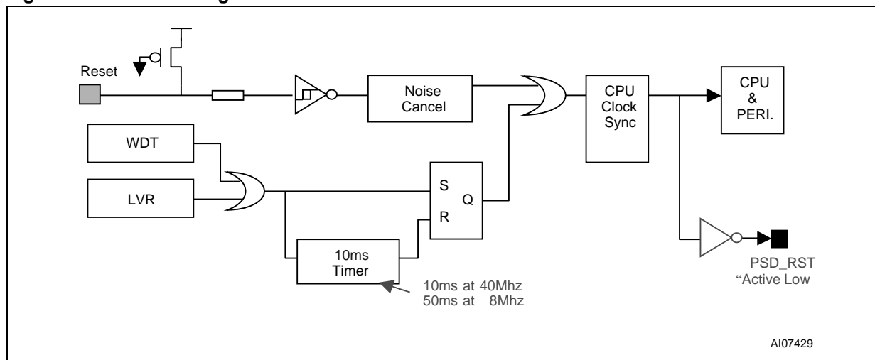
Figure 20. RESET Configuration
