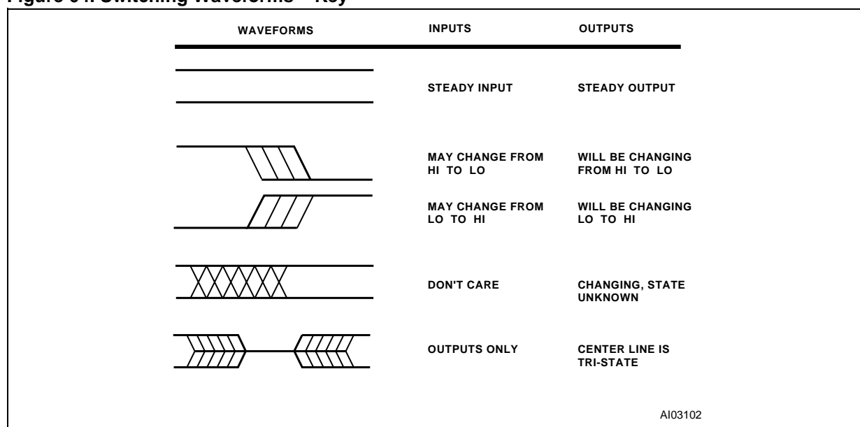
Figure 64. Switching Waveforms – Key
