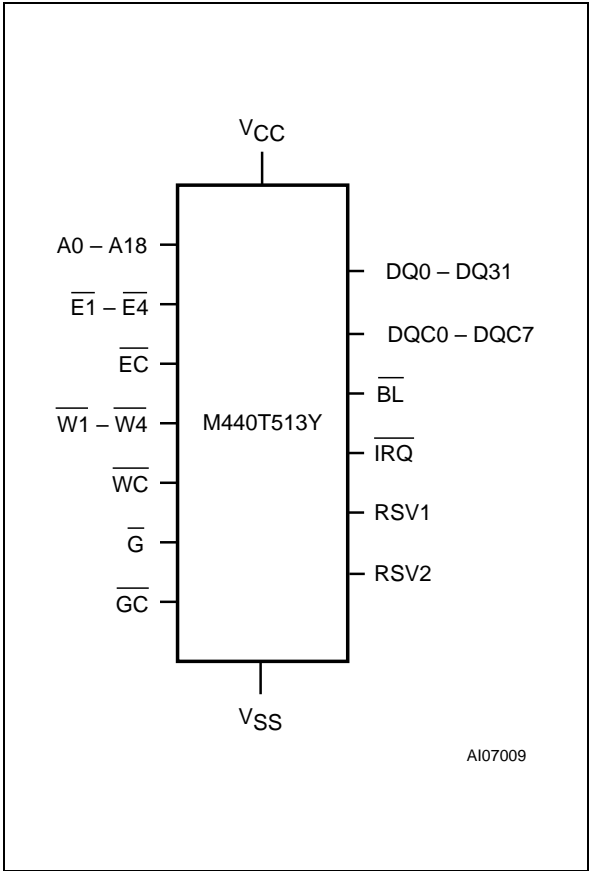
Figure 2. Logic Diagram
