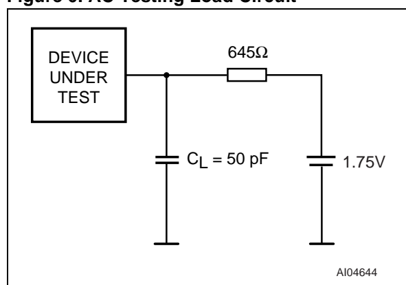
Figure 6. AC Testing Load Circuit
