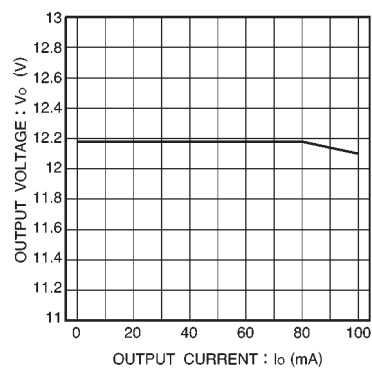
Fig.7 Output characteristic
