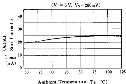
Output Sink Current 2 vs. Temperature
