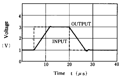
Pulse Response ( V^+ = 15V, R_L = 2k\Omega )
