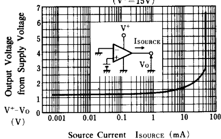
Output Source Current ( V^+ = 15V )
