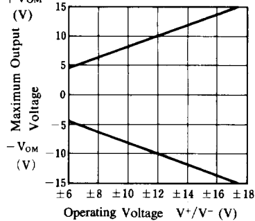
Maximum Output Voltage Swing vs. Operating Voltage
