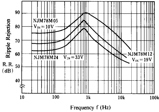
NJM78M05/12/24 Ripple Rejection
