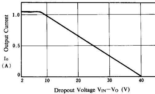
NJM78M00 Series Short Circuit Output Current
