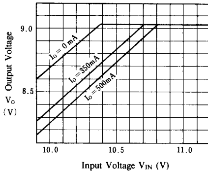
NJM78M09 Dropout Characteristics
