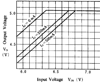
NJM78M05 Dropout Characteristics
