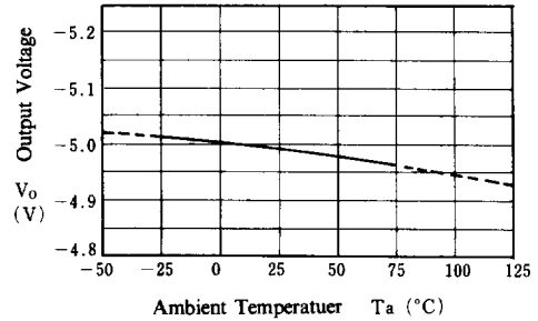
NJM7905 Output Voltage vs. Temperature
