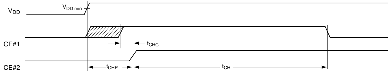
Figure 34. Power-on Timing
