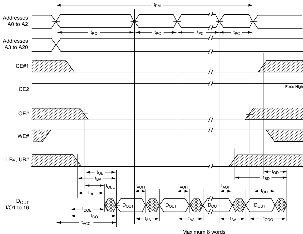
Figure 29. Page Read Timing
