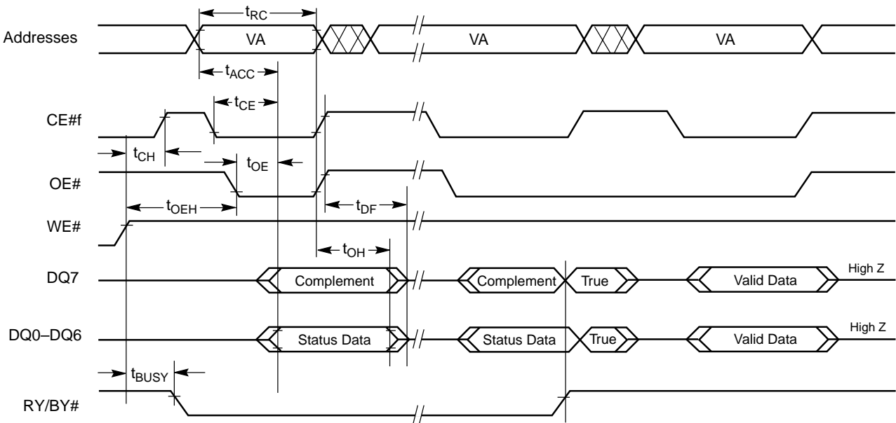
Figure 21. Back-to-back Read/Write Cycle Timings
