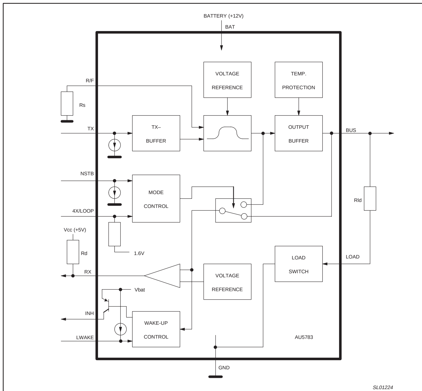
Figure 1. Block diagram
