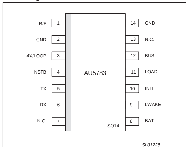
Figure 2. Pin configuration
