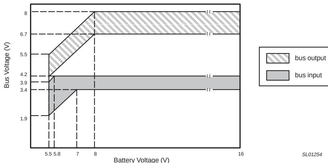
Figure 3. Bus voltage vs battery voltage
