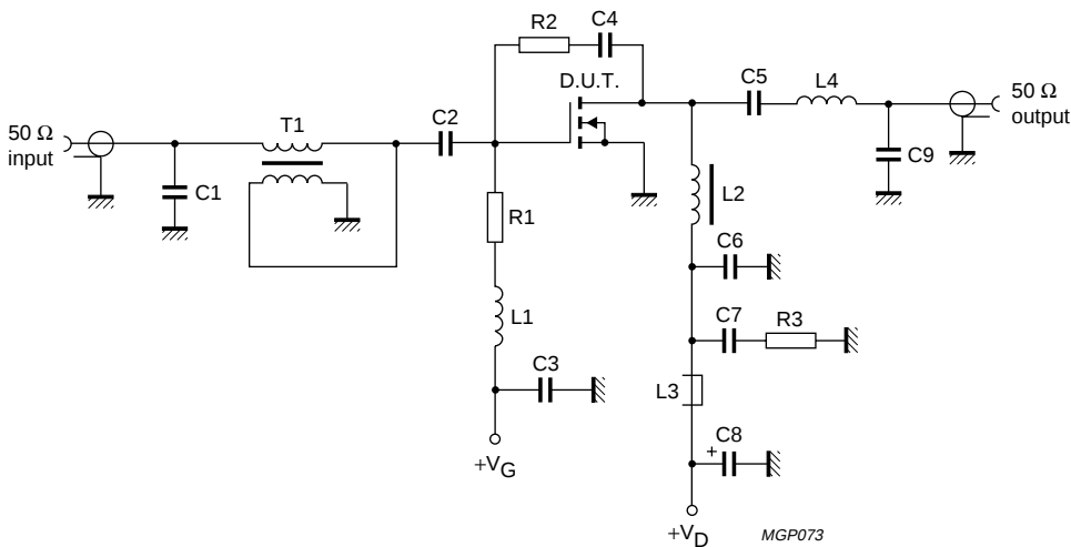
Fig.13 Test circuit for class-A operation.
