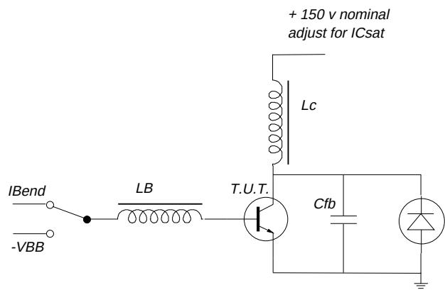
Fig.3. Switching times test circuit.
