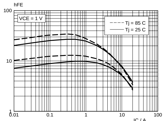
Fig.4. High and low DC current gain. h_{FE} = f(I_C) V_{CE} = 1 \text{ V}
