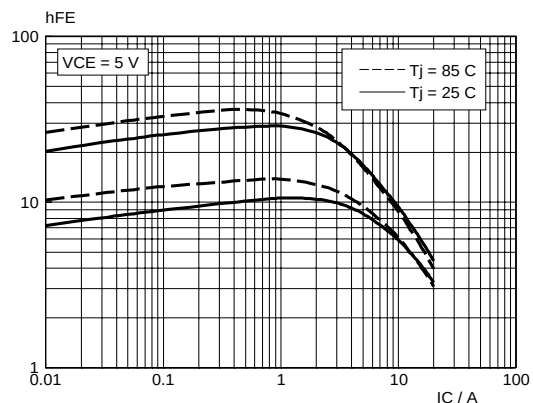
Fig.5. High and low DC current gain. h_{FE} = f(I_C) V_{CE} = 5 \text{ V}
