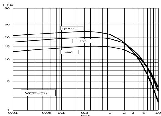
Fig. 9. Typical DC current gain. h_{FE} = f(I_C) parameter V_{CE}
