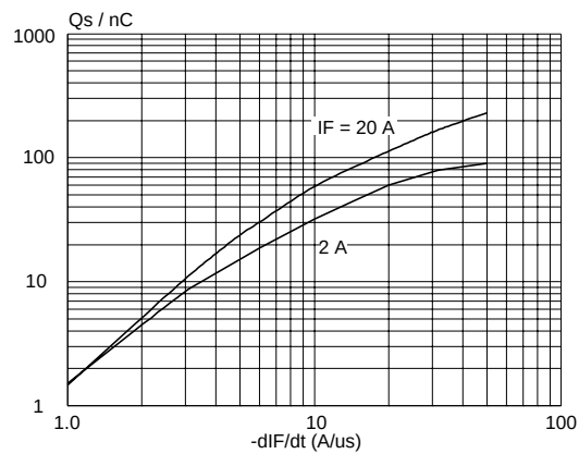
Fig.8. Maximum Q_s at T_j = 25^\circ\text{C}
