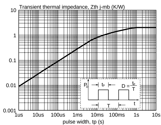
Fig.9. Transient thermal impedance Z_{th} = f(t_p)
