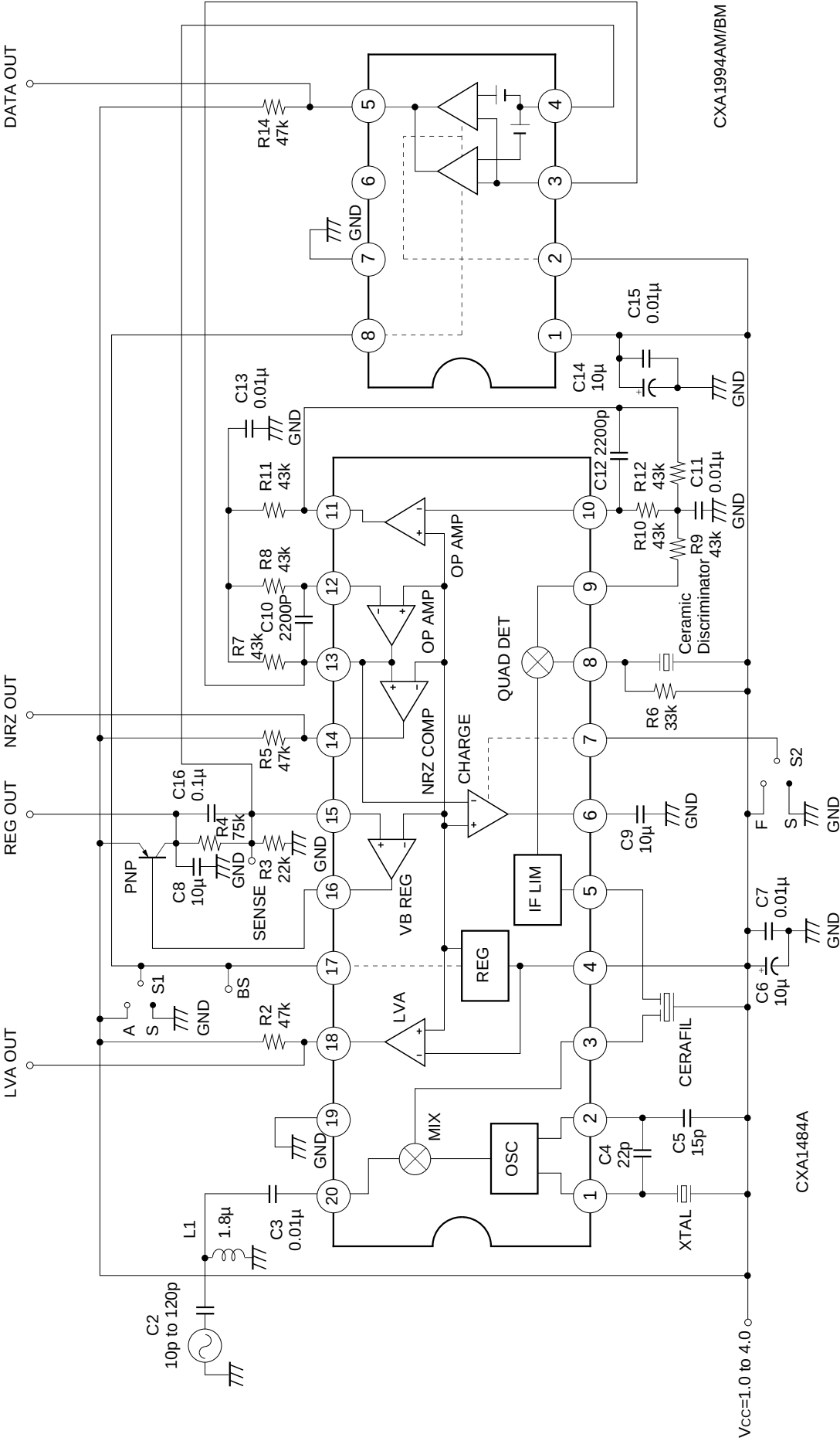
Application Circuit
