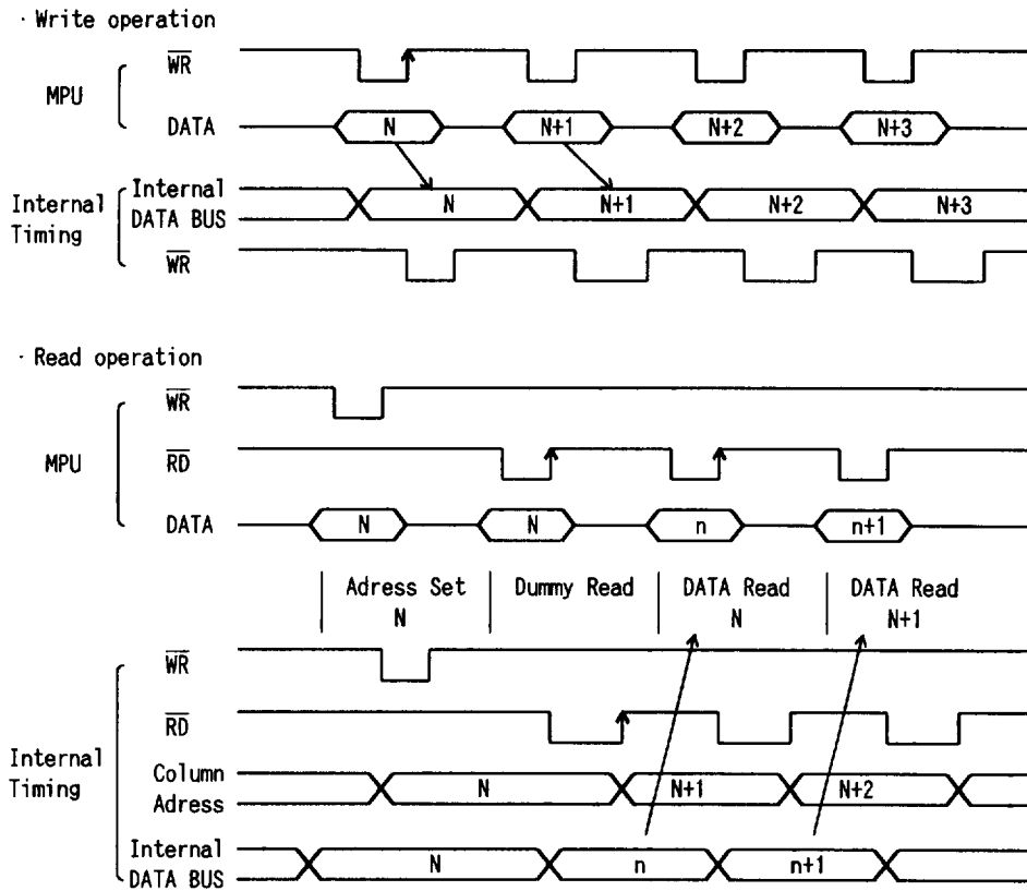
Fig.2 MPU Interface Timing
