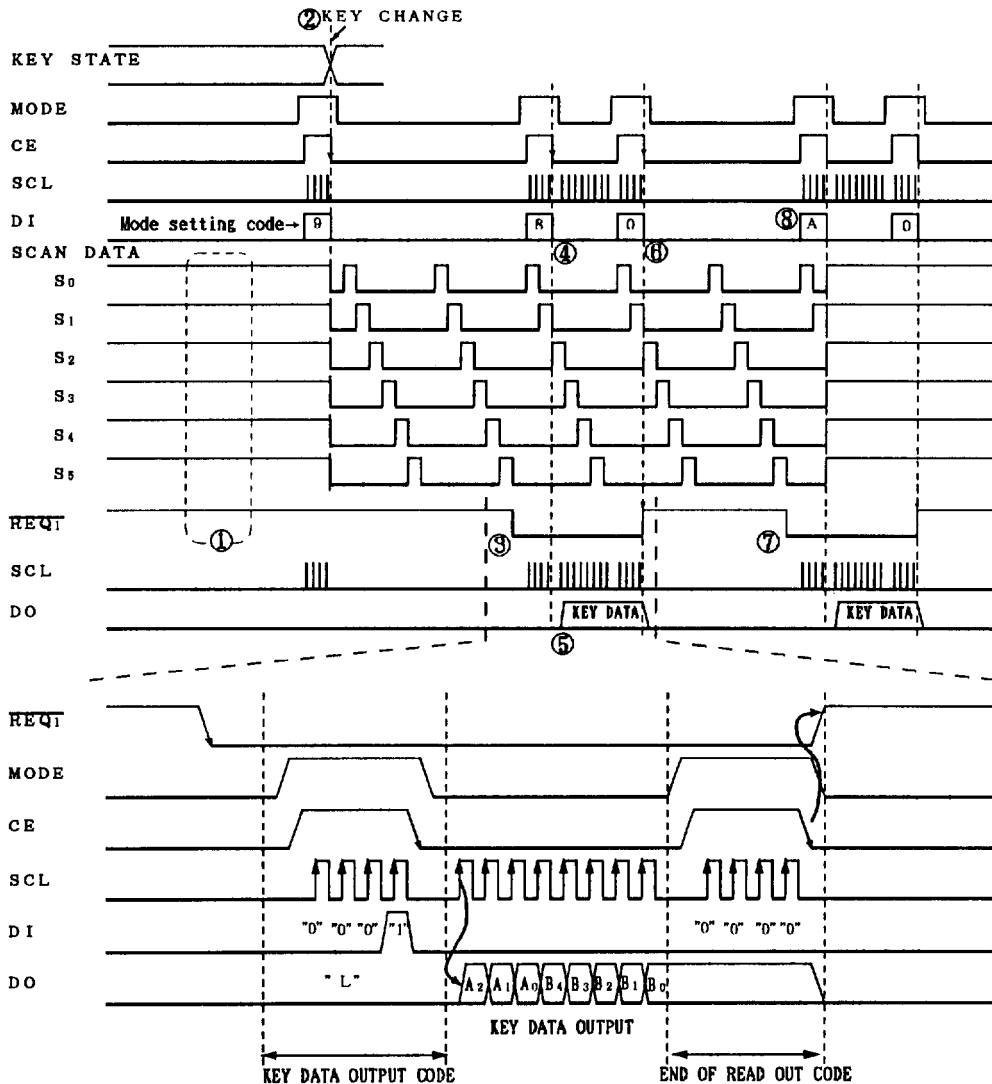
(3-3) Key Scan Timing Chart
